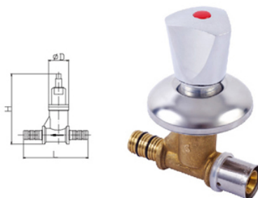
Shutoff Valve Concealed Lockshield · 暗装截止阀
