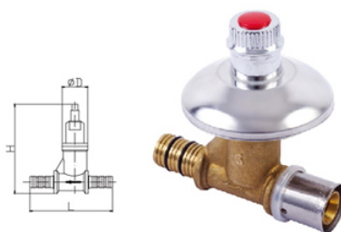
Shutoff Valve Concealed Lockshield · 暗装截止阀
